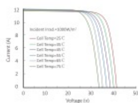
Current-Voltage Curve (LR4-60HPH-365M)
