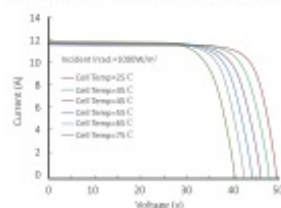
Current-Voltage Curve (LR4-72HPH-440M)
