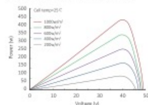
Power-Voltage Curve (LR4-72HPH-440M)
