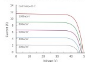
Current-Voltage Curve (LR4-72HPH-440M)
