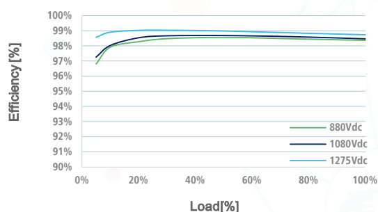
Efficiency Curve
