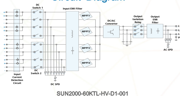
Circuit Diagram
