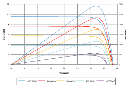
Current-Voltage & Power-Voltage Curve (290-20)
