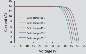
Current-Voltage (565W)
