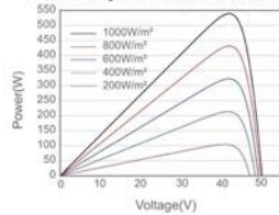
Power-Voltage Curve JAM72S30-540/MR/1500V
